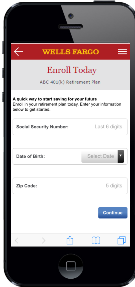
Login screen
